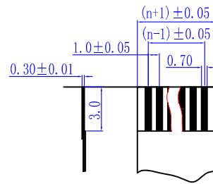
FFC/FPC Dimension
