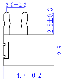
FFC/FPC Dimension
